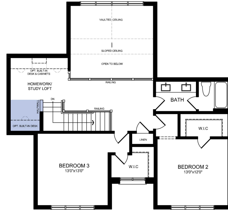
SECOND FLOOR PLAN MODERN CRAFTSMAN ELEVATION
