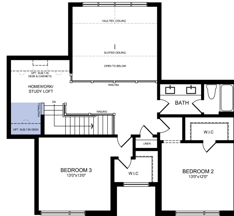
SECOND FLOOR PLAN CONTEMPORARY ELEVATION
