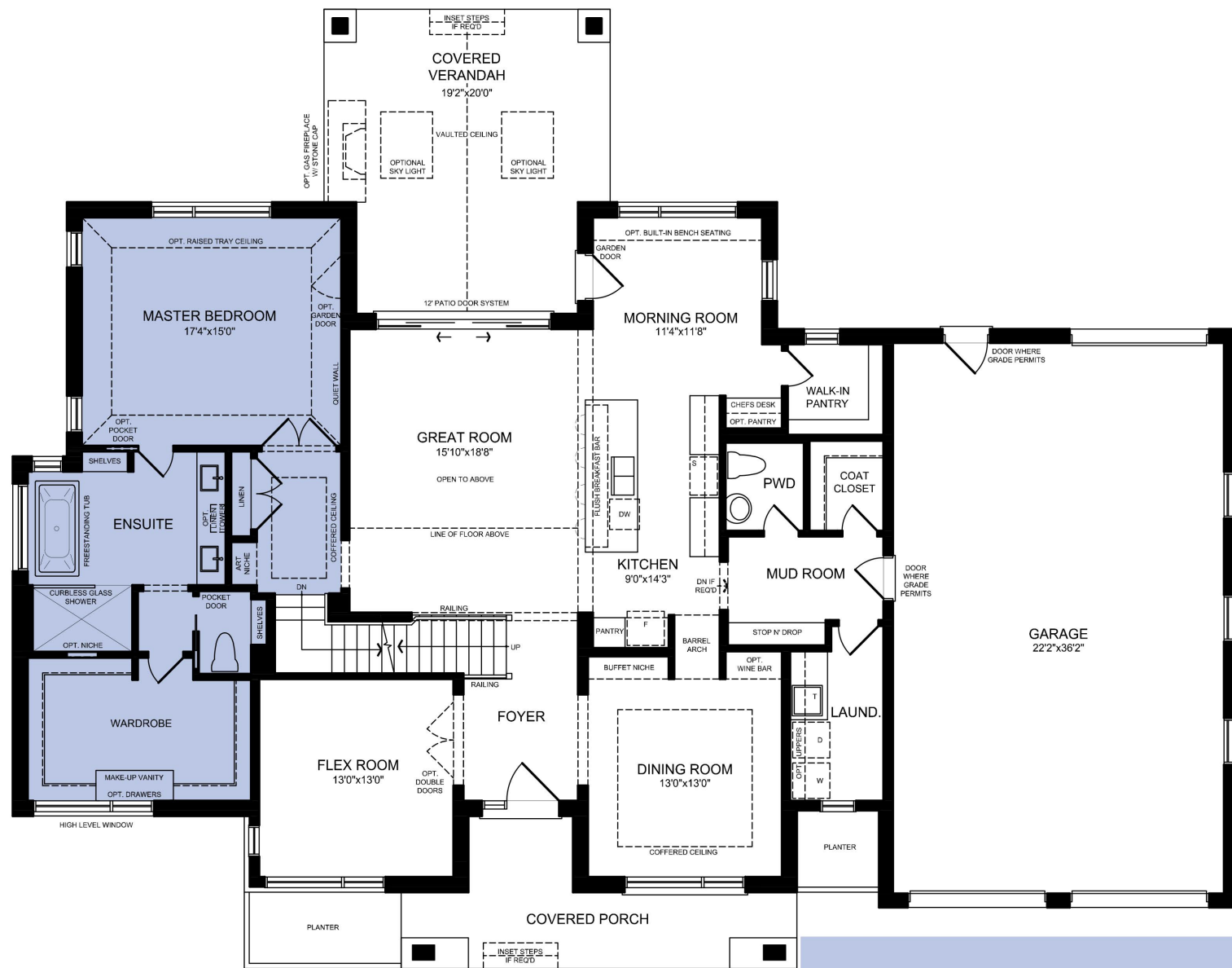
MAIN FLOOR PLAN CONTEMPORARY ELEVATION
