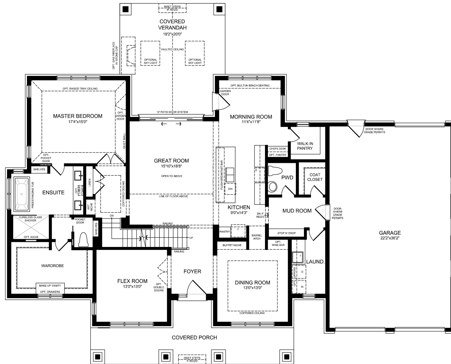
MAIN FLOOR PLAN MODERN CRAFTSMAN ELEVATION
