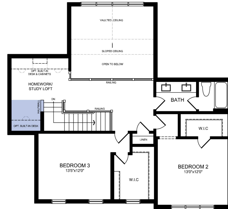
SECOND FLOOR PLAN MODERN FARMHOUSE ELEVATION
