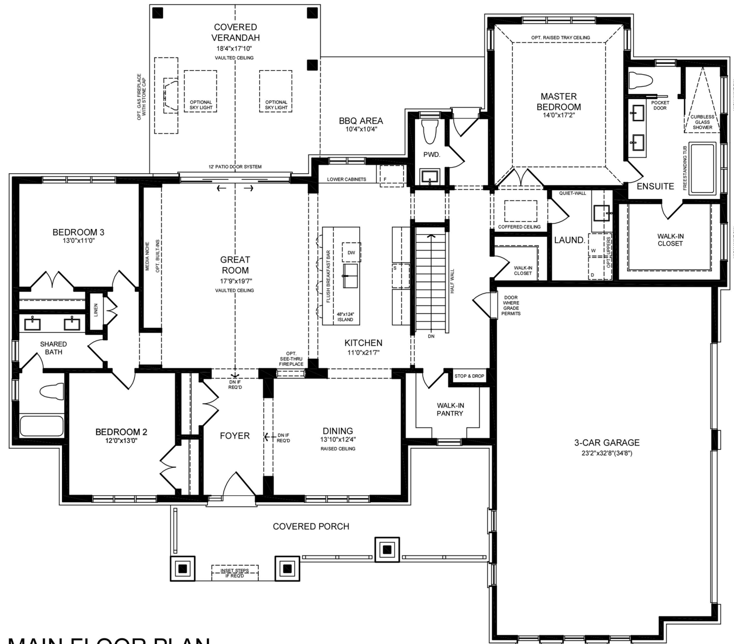
MAIN FLOOR PLAN MODERN CRAFTSMAN ELEVATION
