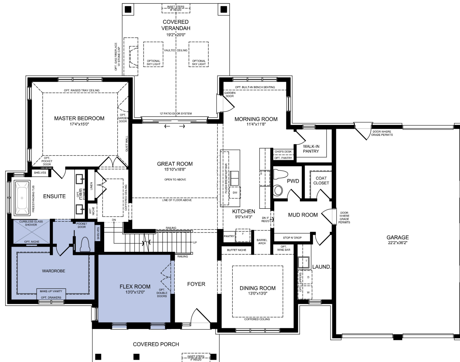
MAIN FLOOR PLAN MODERN FARMHOUSE ELEVATION
